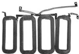
132392 Field Coil
