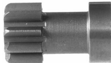
134180 # Dp Gear ID 11.90, OD 25.30, Height 44.40, No./ teeth 9
