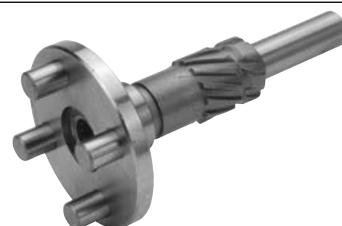
237842 Gear Shaft Servicing: M009T80472, M009T80473, M009T83671, M9T80472, M9T80473, M9T83671 Total length 125.60, No./ splines 12
