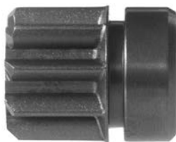
134168 Dp Gear ID 12.00, OD 25.10, Height 31.90, No./ teeth 9
