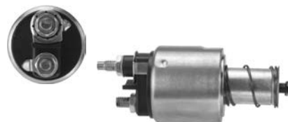
239966 Solenoid Replacing: 594459 Servicing: d7e52 12 V, B+ M8, OD 54.00, Total length 97.07, Height/ B+ 18.00, No./ terminals 2
