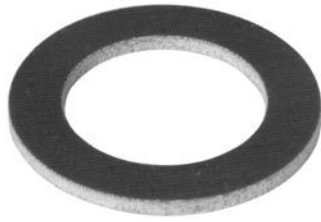
134765 DP Washer ID 31.35, OD 47.85, Thickness 2.55
