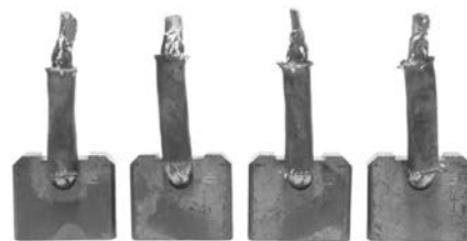
140361 Brush Set
