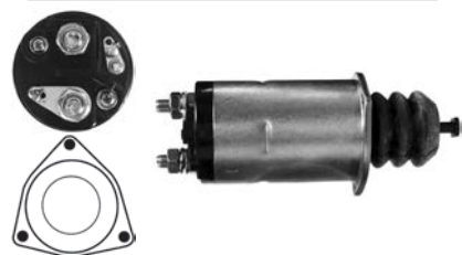
231734 Solenoid
