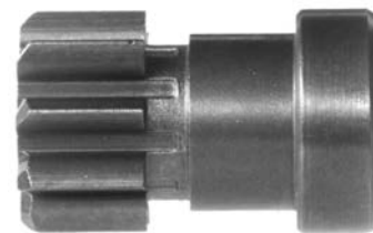
134181 Dp Gear ID 11.80, OD 25.50, Height 41.45, No./ teeth 9
