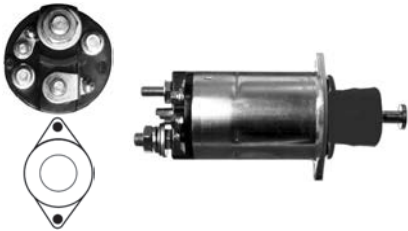
135677 Solenoid
