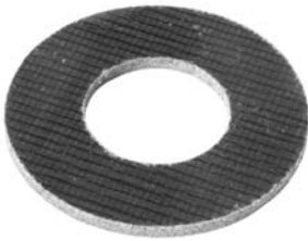
134759# DP Washer ID 28.85, OD 60.35, Thickness 3.20
