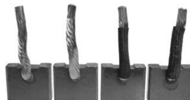
140395 Brush Set
