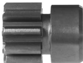
134192 Dp Gear ID 14.00, OD 34.00, Height 42.45, No./ teeth 9
