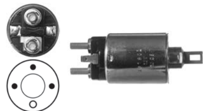
131802 Solenoid Replacing: md607933, m371x82373, m371x81871, m371x81371, m371x80571, m371x55072, m371x55071, m371x54871 Servicing: M001T50471, M002T10171, M002T10271, M002T20181, M002T20181A, M002T20182, M002T20281, M002T23181, M002T50581, M002T50981 12 V, B+ M8, Kl. 50 6.30, OD 51.30, OD/ cover 44.75, Total length 131.00, Height/ B+ 18.25, Width/ kl. 50 15.10, Coil bolt M8, Coil bolt 2 18.25, No./ terminals 3 Cap: HC-CARGO 133273.
