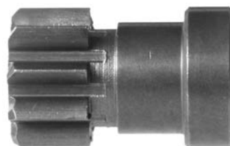
134184 # Dp Gear ID 11.90, OD 28.95, Height 47.25, No./ teeth 9
