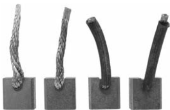
140337 Brush Set
