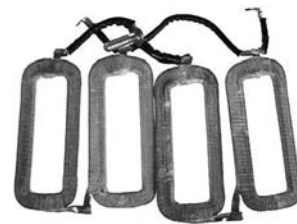
130954# Field Coil
