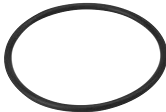
235692 O-ring ID 44.00, Thickness 2.45, Material Rubber
