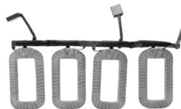
135200 Field Coil
