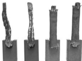
140347 Brush Set
