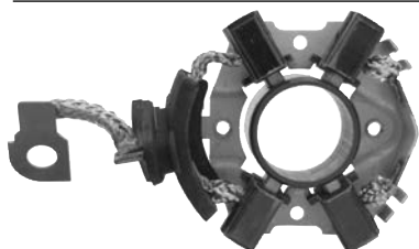
235531 Brush Gear
