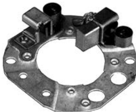
138534 Brush Gear
