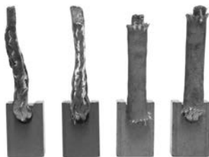
140347 Brush Set
