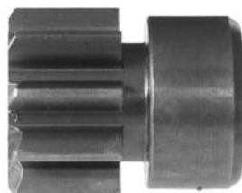
134195 Dp Gear ID 14.30, OD 34.00, Height 42.55, No./ teeth 9
